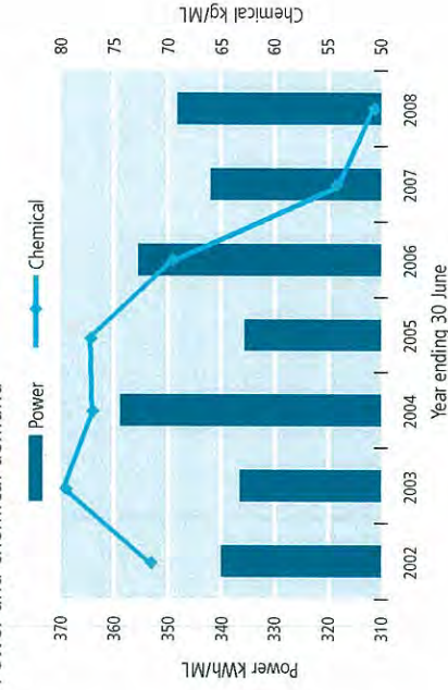
Power and chemical demand
