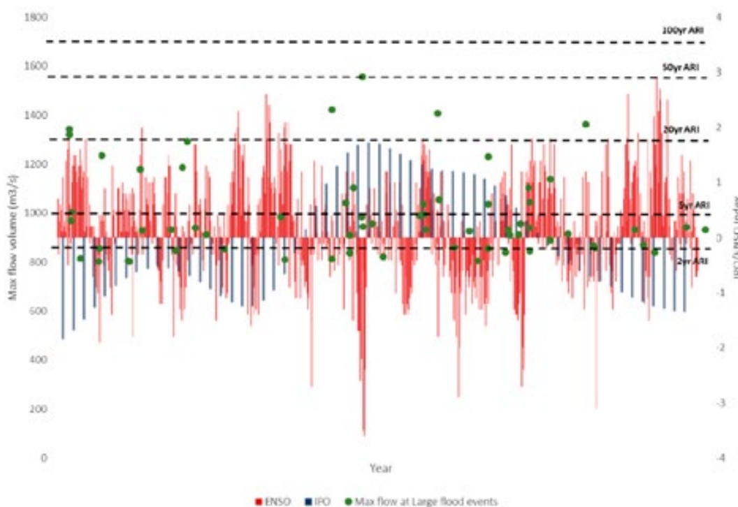
Figure 24: Maximum flood peaks for the 50 largest recorded floods in the Waiōhine River Catchment are shown as green dots, El Nino Southern Oscillation (ENSO) cycles are shown in red, IPO cycles are in blue. Tonkin and Taylor from Creative Commons.
