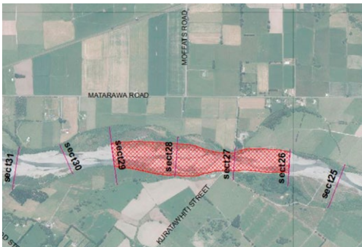
Figure 35: Showing Raised Bed Level At End of Kuratawhiti Street – landriversea Consulting.
